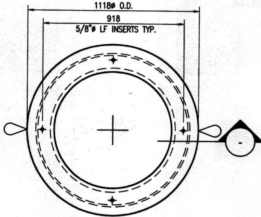
ADAPTOR PLAN
