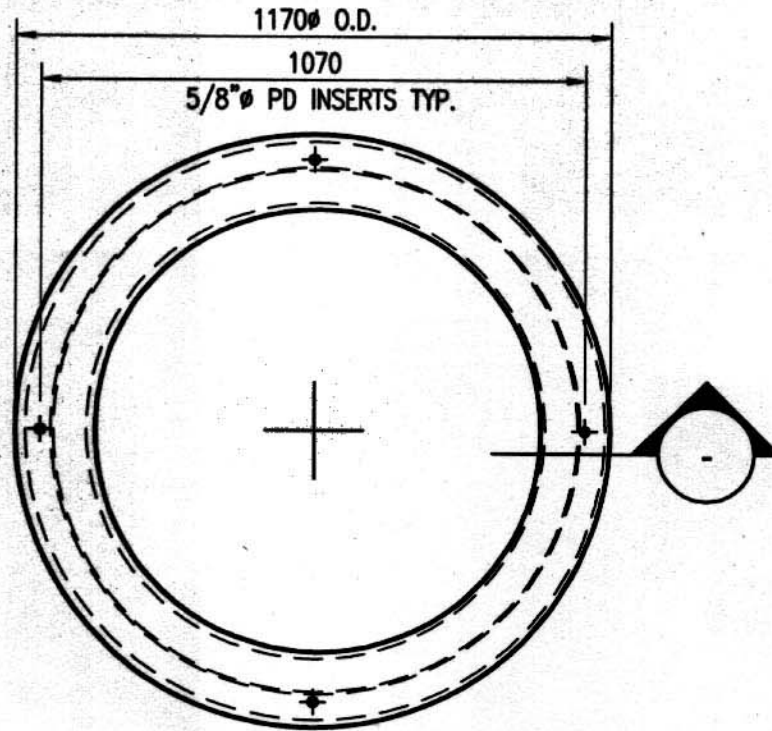
ADAPTOR PLAN
