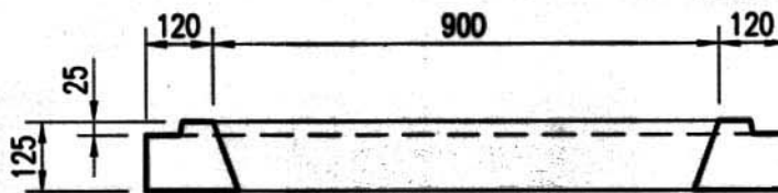
SECTION Mk#: 210-50 MASS: 120 kg (265 lbs)
