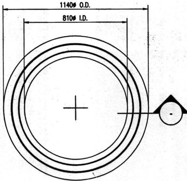
ADAPTOR PLAN
