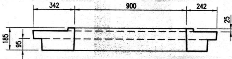
SECTION
