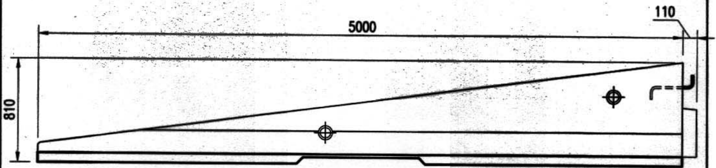
ELEVATION Mk#: 772-03 (Male Transition) WEIGHT: 2065 kg (4555 lbs)
