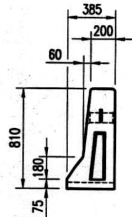
TYP. END VIEW
