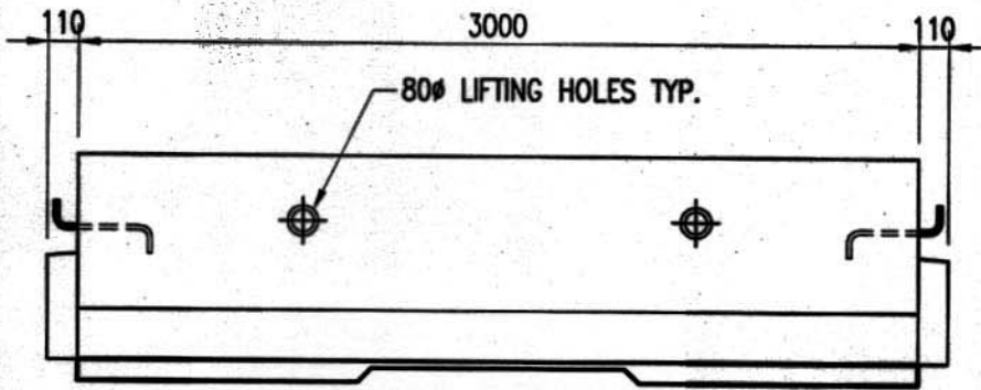
ELEVATION Mk#: 772-01 (Male) WEIGHT: 1525 kg (3365 lbs)
