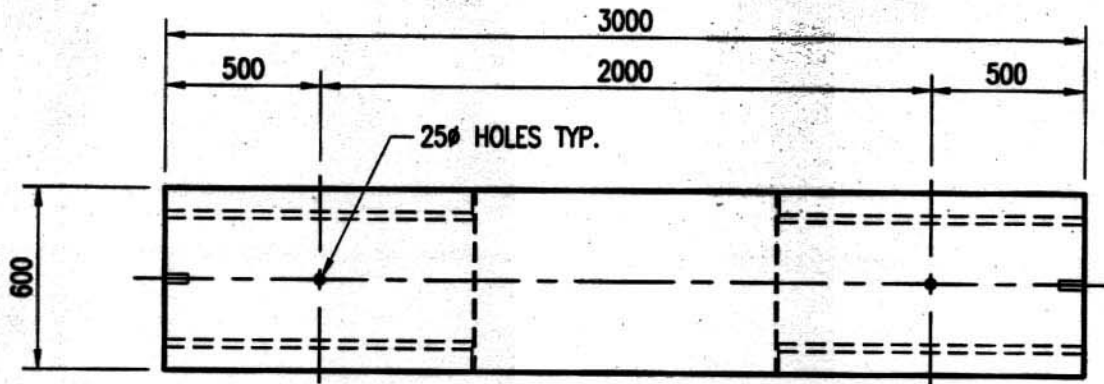
PLAN
