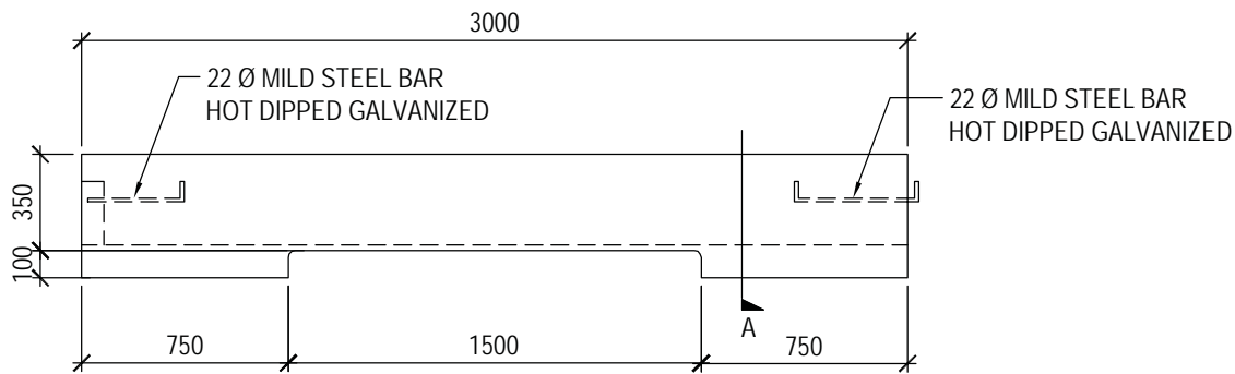
SIDE ELEVATION
