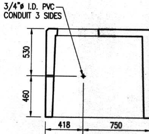
A SECTION
